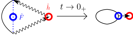
Figure 6: Schematic path-integral diagram of Eq. (121) with the imaginary time path shown as a curved line, the real time path with a wavy line and the flux and side operators as blue and red circles respectively. Placing the flux operator at the average of the forward and backward real-time paths (left) leads to the flux and side dividing surfaces being in the same place in path-integral space in the t \rightarrow 0_+ limit (right).
