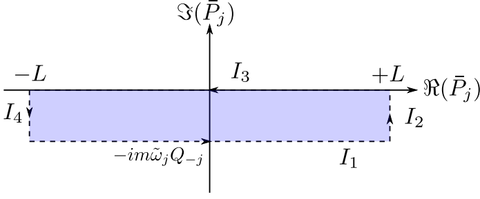
Figure 4: The contour integral in Eq. (76) in the real and imaginary plane of \bar{P}_j , in the limit L \rightarrow \infty . Matsubara dynamics evaluates the contour I_1 , which is real in P_j but complex in \bar{P}_j , and is the contour given in Eq. (76). This is equivalent to -I_3 , the integral in Eq. (78), provided that I_2 and I_4 vanish and that the region enclosed by the contours (shaded blue box, colour online) is holomorphic (free from singularities). This can easily be shown to hold at t = 0 , giving Eq. (78). At finite time the shaded region is holomorphic for any analytic Hamiltonian [59], and I_2 and I_4 can be shown to be zero in a large variety of limits [59], but their evaluation for an arbitrary potential is challenging [62] and here they are assumed to be zero.
