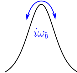
Figure 8: Schematic diagram showing the imaginary mode at the top of the barrier, which would be a saddle point on a multidimensional potential energy surface.
