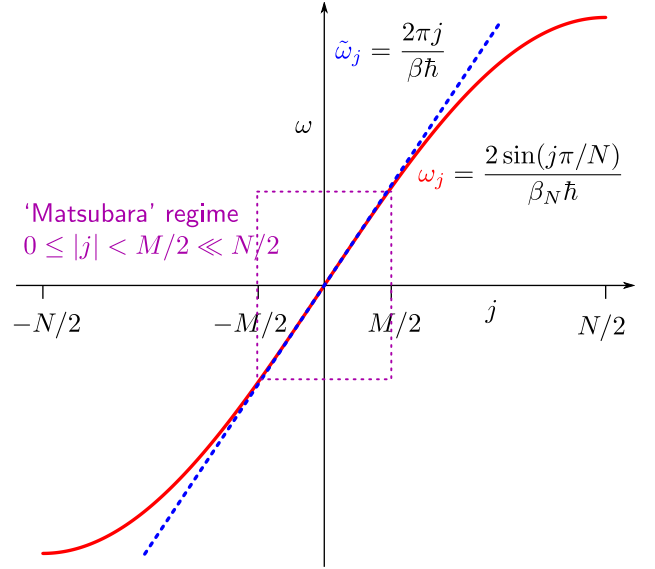
Figure 3: Illustrating how the Matsubara modes \tilde{\omega}_j approximate ring polymer modes \omega_j provided M \ll N .
