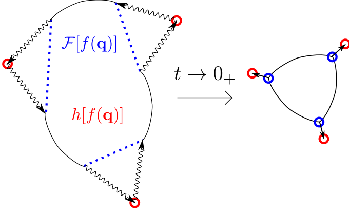
Figure 7: Schematic diagram of the Generalized Kubo correlation function in Eq. (128) for the case of N = 3 , with a generalized dividing surface f(\mathbf{q}) and \mathcal{F}[f(\mathbf{q})] = \delta[f(\mathbf{Q})]S(\mathbf{P}, \mathbf{Q}) is the flux through f(\mathbf{q}) at t = 0 . In the t \rightarrow 0_+ limit (and for N \rightarrow \infty ), the ‘stretches’ in the ring polymer can be integrated out leading to the ring-polymer flux, shown on the right.
