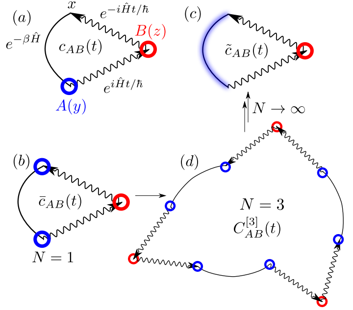
Figure 1: Different forms of quantum mechanical correlation functions discussed in this article. The imaginary time path shown as a curved line, the real time path with a wavy line and the \hat{A} and \hat{B} operators as blue and red circles respectively. (a) is the conventional asymmetric-split correlation function, (b) one form of symmetric splitting, (c) the Kubo-transformed function (with the operator \hat{A} ‘smeared’ along the imaginary time trajectory). The Generalized Kubo transformed function (d) is obtained by polymerising (b), and is equivalent to the conventional Kubo transformed function (c) in the N \rightarrow \infty limit for linear operators.
