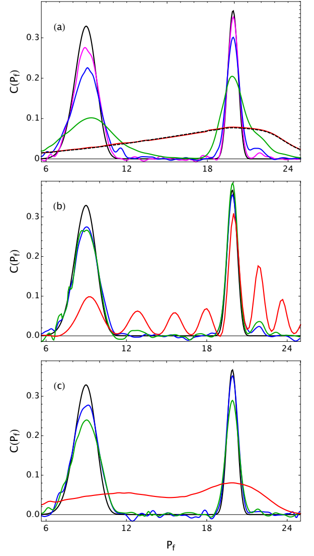
FIG. 3. The distribution of final nuclear momentum with model 2 and incident energy of 0.1 E_h . The exact quantum result (black, solid) is shown in each panel along with (a) the Husimi-IVR (black, dashed) and MQC-IVR where each dof is treated with the same filtering strength: c = 0.01 (pink), c = 0.05 (blue), c = 0.1 (green), and c = 10.0 (red); (b) the MQC-IVR results where the nuclear filtering parameters are fixed near the quantum limit, c_{\text{nuc}} = 0.01 , and the electronic filtering parameters are varied from c_{\text{el}} = 0.05 (blue) to c_{\text{el}} = 0.1 (green) and c_{\text{el}} = 10.0 (red); (c) MQC-IVR results where the electronic filtering parameters are fixed in the quantum-limit, c_{\text{el}} = 0.01 , and the nuclear filtering parameters are varied from c_{\text{nuc}} = 0.05 (blue) to c_{\text{nuc}} = 0.1 (green) and c_{\text{nuc}} = 10.0 (red).
